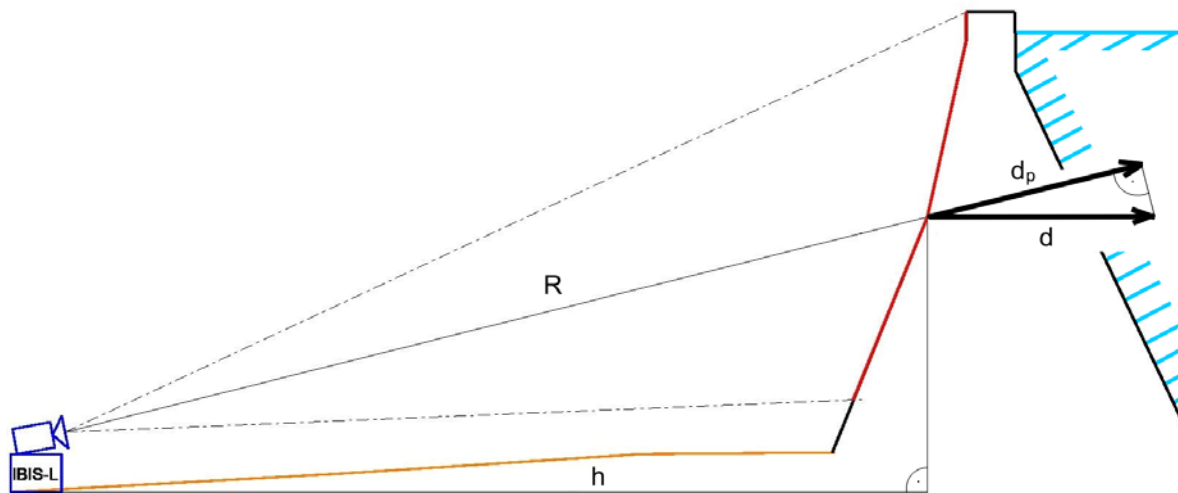
Fig. 4 Line of sight movement ( d_p ) and real movement ( d )
