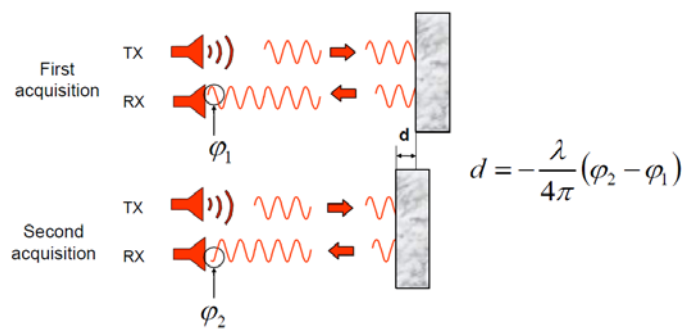
Fig. 3 Radar interferometry principle
