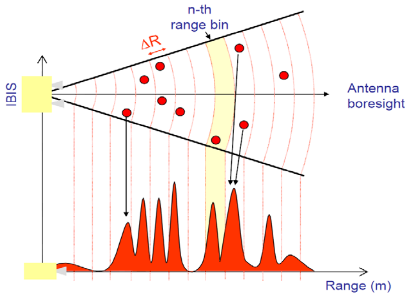
Fig. 1 Range resolution concept
