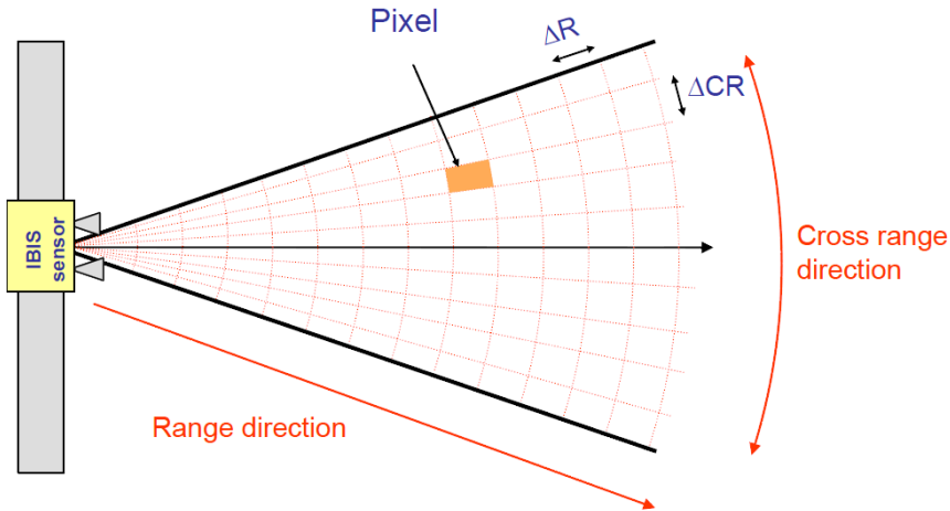
Fig. 2 Resolution grid example
